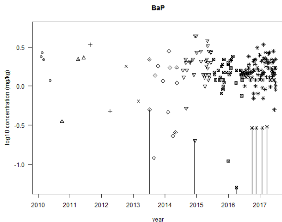
Figure B1-4: Benzo[a]pyrene. Log10 concentration against year of sampling. Different symbols indicate different year of sampling. All samples taken at a granules production site. Samples taken from (aged) sports pitches are not included. Vertical lines indicate that <LOD was measured. The concentration at the upper end of the vertical line is the LOD.
