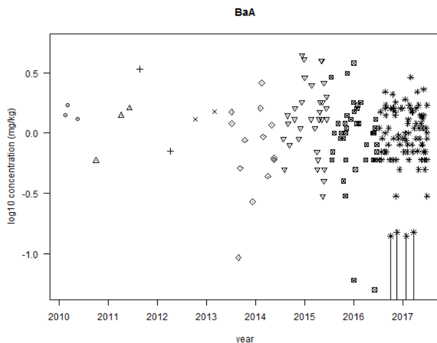
Figure B1-2: Benzo[a]anthracene. Log10 concentration against year of sampling. Different symbols indicate different year of sampling. All samples taken at a granule production site. Samples taken from (aged) sports pitches are not included. Vertical lines indicate that <LOD was measured. The concentration at the upper end of the vertical line is the LOD.
